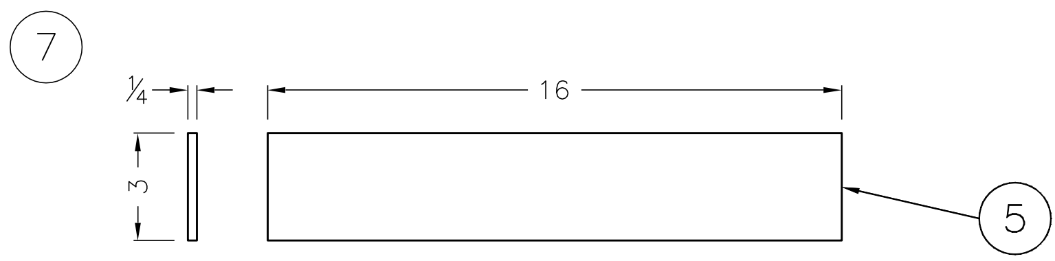
STOP PLATE
