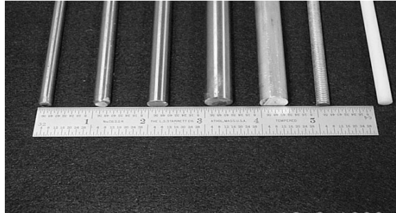
Picture 1: Entire Contents of the Tube (Left to right) Drill Rods ( 5/16''\phi , 3/8''\phi , 1/4''\phi , 1/2''\phi )(2 of each), Aluminum Rod ( 1/2''\phi )(2), Threaded Rod ( 1/4''\phi ) (1), and Delrin (Acetal) Rod ( 1/4''\phi ) (1)
