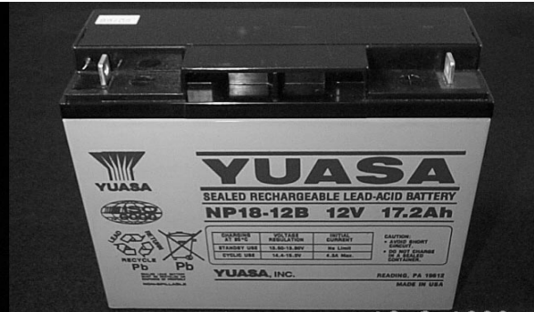
Picture 4: Battery (2)
